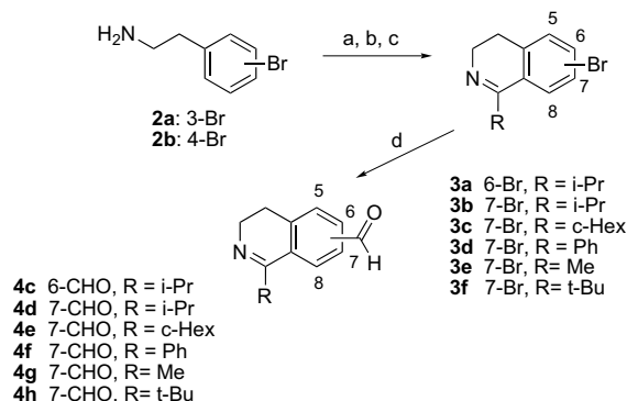
Scheme 1. Reagents and conditions: (a) \text{RC(=O)Cl} , \text{Et}_3\text{N} ; (b) (\text{COCl})_2 , \text{FeCl}_3 , chloroform; (c) \text{HCl} ; (d) \text{BuLi} , DMF, THF, -78^\circ\text{C} .
