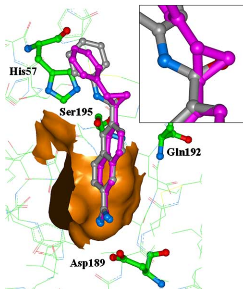
Figure 1. Crystal structure of compound 19a (pink, cyclopropyl link, PDB entry 1U6Q) bound to urokinase is shown overlaid with compound 1a (grey, amide link, PDB entry 1OWE). His57, Asp189, Gln192 and Ser195 are shown in thick bonds. The surface of the S1 pocket is shown. The inset shows a close-up view of the cyclopropyl/amide overlay.
