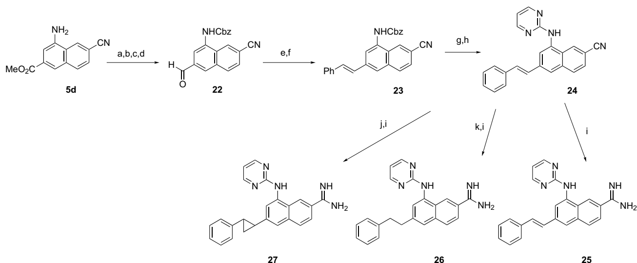
Scheme 3. Reagents and conditions: (a) Cbz-Cl, i -PrNEt 2 , THF; (b) LiOH, dioxane, H 2 O; (c) (COCl) 2 , THF; (d) LiAl(O t Bu) 3 H, THF, −78 °C; (e) Ph 3 PCH 3 Br, NaHMDS, THF; (f) PhN 2 BF 4 , Pd 2 (dba) 3 , DMF; (g) Ba(OH) 2 , DME, 70 °C; (h) 2-Br-pyrimidine, Pd 2 (dba) 3 , NaO t Bu, toluene; (i) AlMe 3 , NH 4 Cl, toluene; (j) CH 2 N 2 , Pd(OAc) 2 , THF, ether; (k) Pd/C, H 2 , MeOH.
