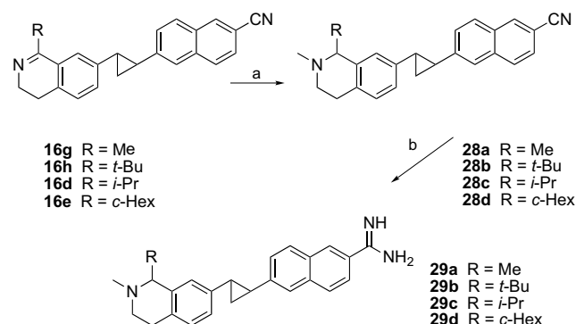
Scheme 4. Reagents and conditions: (a) NaBH 3 CN, CH 2 O, MeOH; (b) LiHMDS, THF, HCl.
