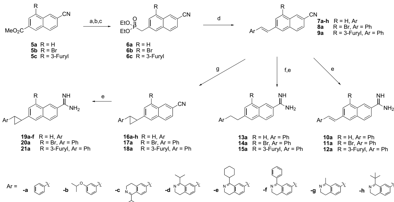
Scheme 2. Reagents and conditions: (a) \text{NaBH}_4 , \text{CaCl}_2 , \text{EtOH} ; (b) \text{PPh}_3 , NBS, dichloromethane; (c) \text{P(OEt)}_3 , 130^\circ\text{C} ; (d) \text{LiHMDS} , \text{ArCHO} 4a–h , THF; (e) \text{LiHMDS} , THF, \text{HCl} ; (f) \text{Pd/C} , \text{H}_2 , \text{MeOH} ; (g) \text{CH}_2\text{N}_2 , \text{Pd(OAc)}_2 , THF, ether.
